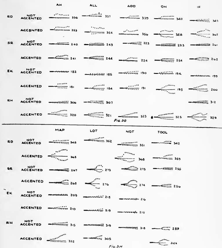
FIG. 3 (Continued). Tracings of oscillograms of speech sounds.
